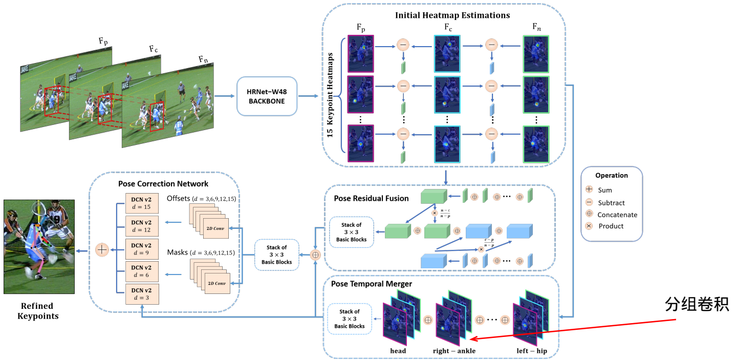
Figure 2. Overall pipeline of our DCPose framework. The goal is to locate the keypoint positions for the current frame F_c . First, an individual person i is assembled into an input sequence \text{Clip}_i(p, c, n) , and a HRNet backbone predicts initial keypoint heatmaps \mathbf{h}_i(p), \mathbf{h}_i(c), \mathbf{h}_i(n) . Our Pose Temporal Merger (PTM) and Pose Residual Fusion (PRF) networks work concurrently to obtain an effective search scope \Phi_i(p, c, n) and pose residuals \Psi_i(p, c, n) , respectively. These are then fed into our Pose Correction Network (PCN) which refines the keypoint estimation for person i in F_c .
